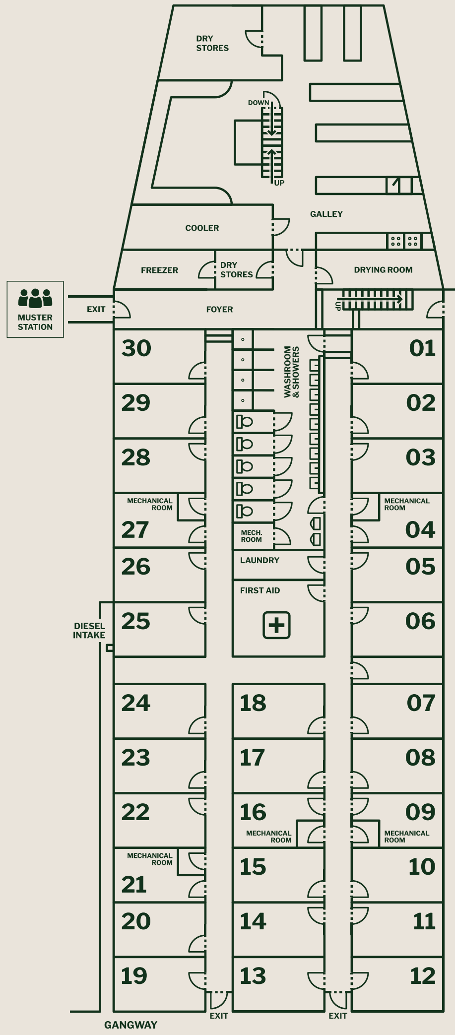
MAIN DECK (LEVEL 2)
